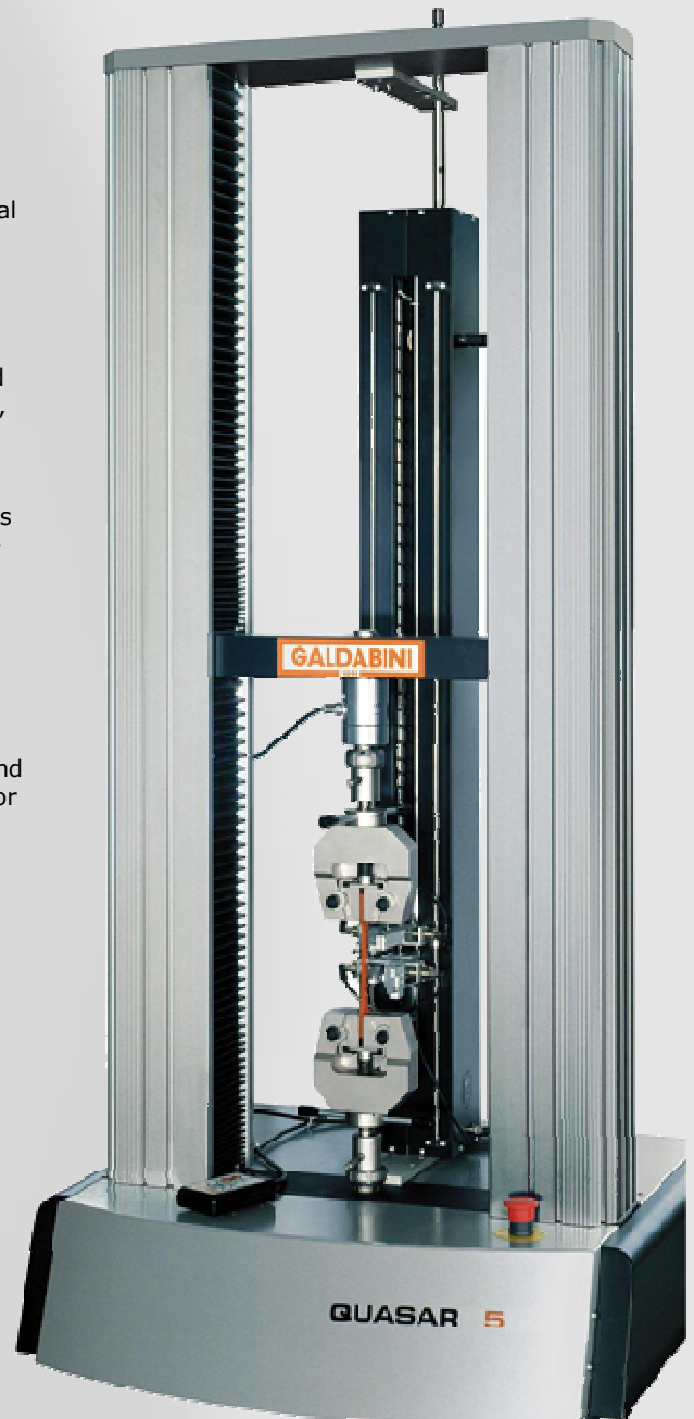
Universal testing machine Quasar 5 with manual wedge grip and "Micron" extensometer
