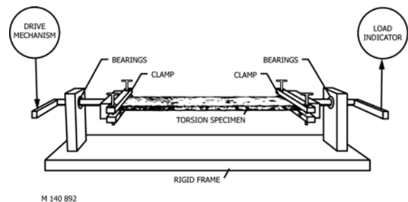
FIG. 11 Fundamentals of a Torsional Test Machine
